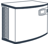
IP0320 W 55.9 • D 62.2 • H 54.6 cm 145 kgs daily at 21/10°C 108 kgs daily at 32/21°C
